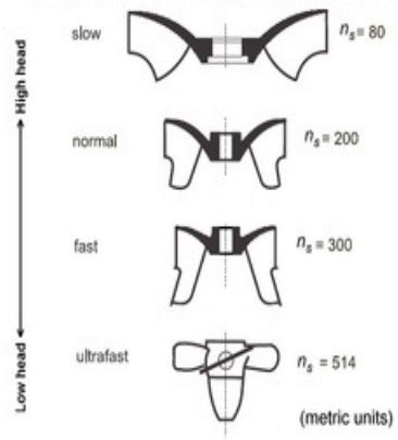
Comparison of Turbine Shape vs. Specific Speed
